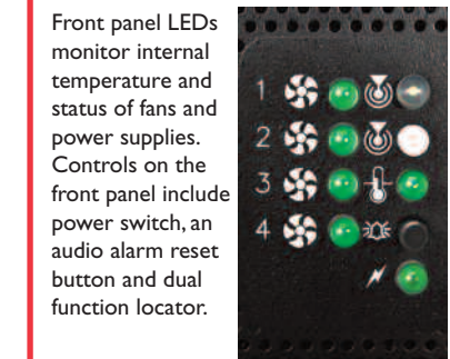
Hot-swappable and hot-plugable redundant power supplies are optimized for high-availability applications.
